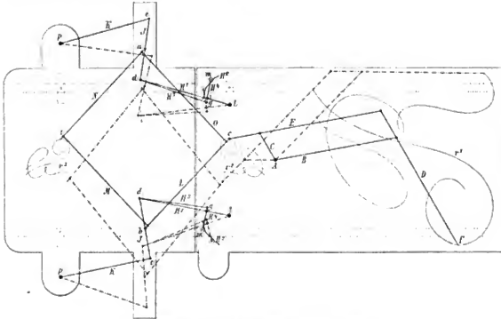
Pannograph von W. Sabel in Koblenz (D. R.-P. Nr. 51.900).
