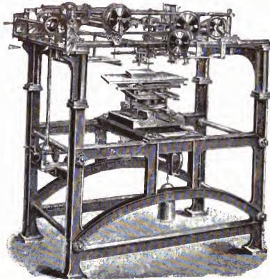
Universal-Gravirmaschine, System Krebs-Lotz.
